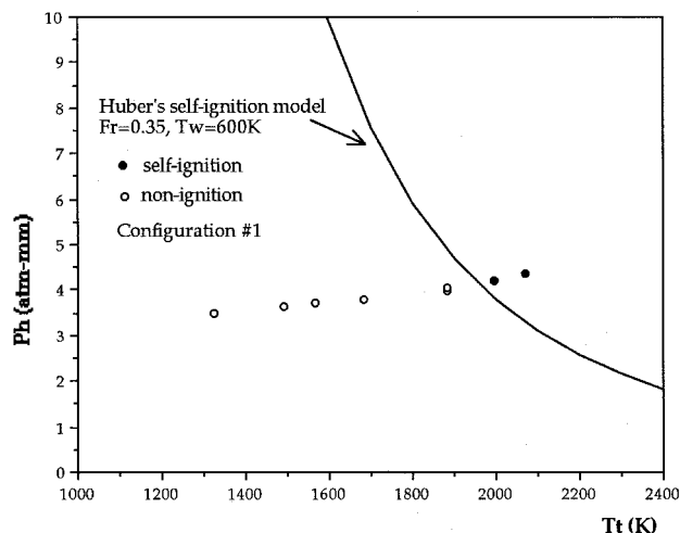
Fig. 4 Self-ignition data in combustor wall configuration no. 1. The uncertainty in T_t is 6.3% for T_t \leq 2000 K, 6.5% for T_t > 2000 K and the uncertainty in Ph is 6.1%.
