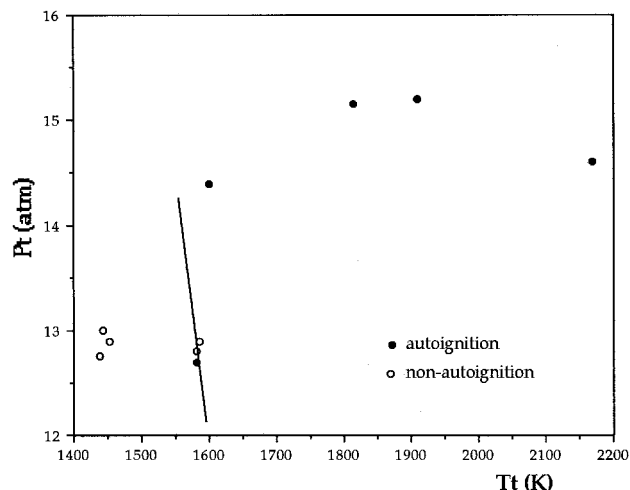
Fig. 7 Self-ignition data in combustor wall configuration no. 2. The uncertainty in T_t is 6.3% for T_t \leq 2000 K, 6.5% for T_t > 2000 K, and the uncertainty in P_t is 6.1%.
