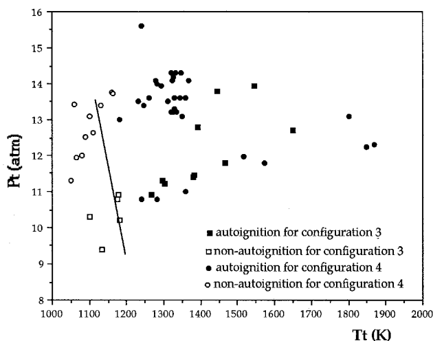
Fig. 8 Self-ignition data in combustor wall configurations no. 3 and no. 4. The uncertainty in T_t is 6.3% for T_t \leq 2000 K, 6.5% for T_t > 2000 K, and the uncertainty in P_t is 6.1%.
